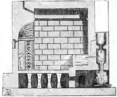
Fig. 393. Hypocaustus of a Roman villa at Tusculum.
